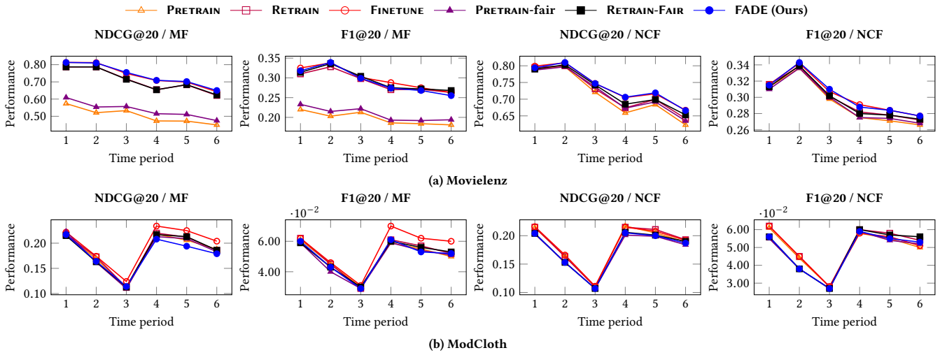
Figure 9: Trend of recommendation performance in Task-N.
