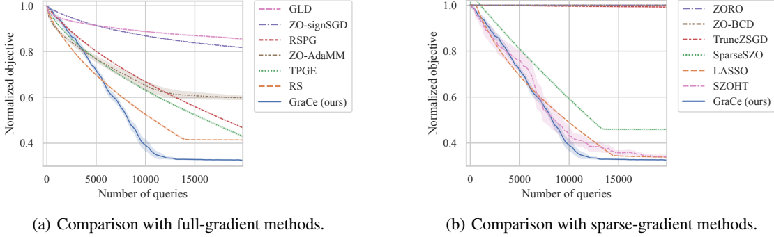
Figure 3. Convergence plots for ATTACK (mean \pm s.e.).
